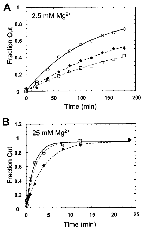
FIGURE 8: Effects of N7-deazaadenosine modification in J3/4 on RNase P ribozyme reaction kinetics. Plot of fraction RNA reacted versus time is shown for unmodified PT50 (circles) and for ribozymes with N7ddA modifications at A62 (diamonds) and A65 (squares). The data are fit to a single-exponential function, as described in Materials and Methods. Panels A and B display data obtained at 2.5 and 25 mM Mg 2+ , respectively.
