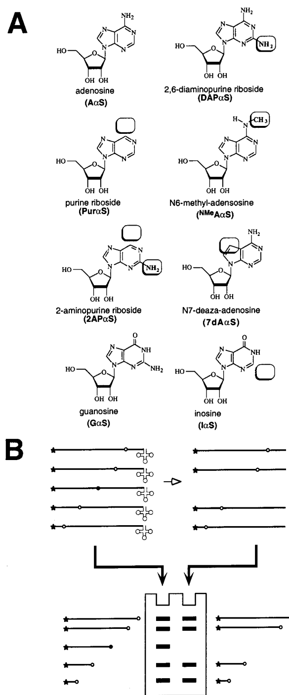
FIGURE 3: Nucleotide analogue interference mapping (NAIM) reagents and selection approach. (A) Chemical structures of the nucleotide analogues employed in these studies. Analogues are shown as nucleosides but are incorporated into RNA as the α-phosphorothioate derivative (26, 75). Base functional groups that are modified relative to adenosine or guanosine are boxed. Abbreviations used in the text and in other figures are shown in parentheses. (B) Diagram of an overview of NAIM as applied using PT332(-5) or PT50. Tethered ribozyme substrate conjugates indicated by a thick straight line with associated cloverleaf tRNA undergo intramolecular cleavage to remove the 3'-terminal tRNA. RNAs are radioactively end-labeled, as indicated by stars and modified internally at on average one modification per RNA, as indicated by circles. Modifications that reduce the rate of self-cleavage, indicated by a filled circle, result in under representation of the modified RNA in the product population. Precursor and product RNAs are isolated and cleaved with iodine at positions of analogue incorporation and visualized by electrophoresis on a standard polyacrylamide sequencing gel.
