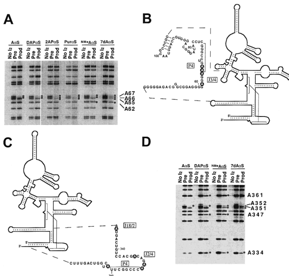
FIGURE 5: Mapping of analogue sensitive positions in the C-domain at low (1.25 mM) Mg^{2+} concentrations. (Panels A and D) Separation of iodine cleavage products of 5'- ^{32}P -end-labeled RNA by polyacrylamide gel electrophoresis. The lane designations are the same as those used in Figure 4. Asterisks indicate the positions where significant interference effects were measured. The individual residue numbers are indicated to the right of the gels. (Panels B and C) Schematic diagrams of the RNase P ribozyme secondary structure. Regions that are mapped in the accompanying gels are highlighted. Individual residues that are sensitive to one or more of the analogues surveyed are circled and the element of RNase P RNA secondary structure in which they are located are indicated in boxes adjacent to the RNA sequence.
